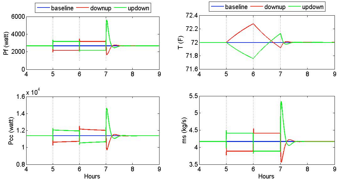
Figure 5. Simulation results for the default case. Plots show comparison among the baseline, the up-down sequence, and the down-up sequence. Upper left: fan power; lower left: cooling power; upper right: room temperature; lower right: supply air flow rate.
